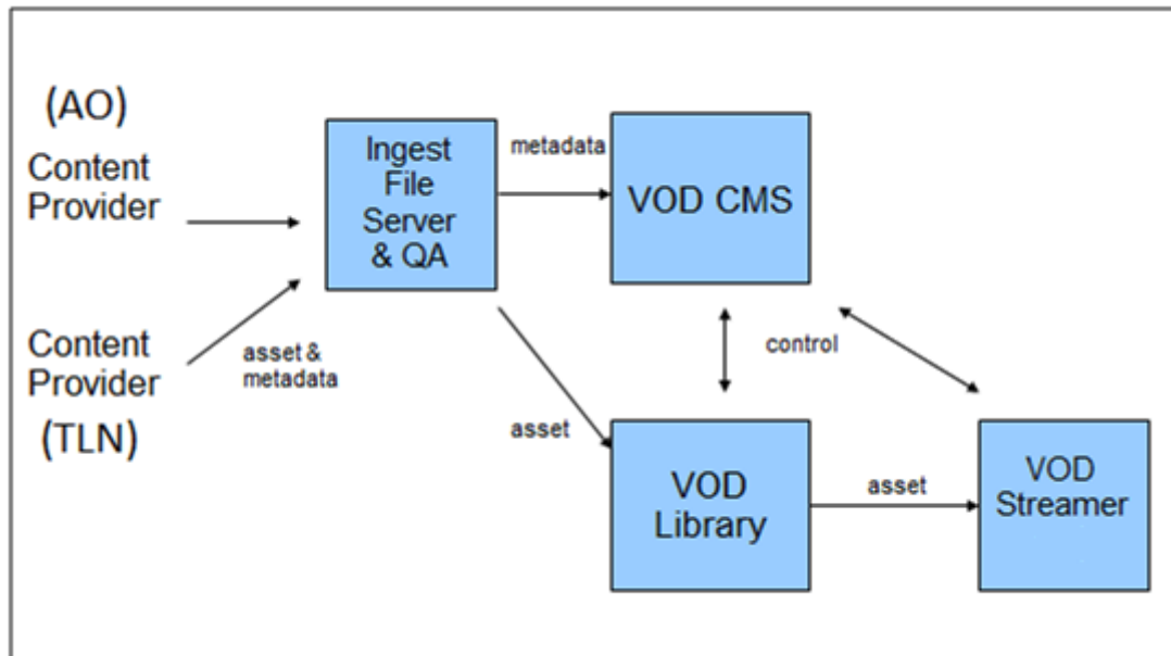
Figure 3-1: VoD CMS Setup
