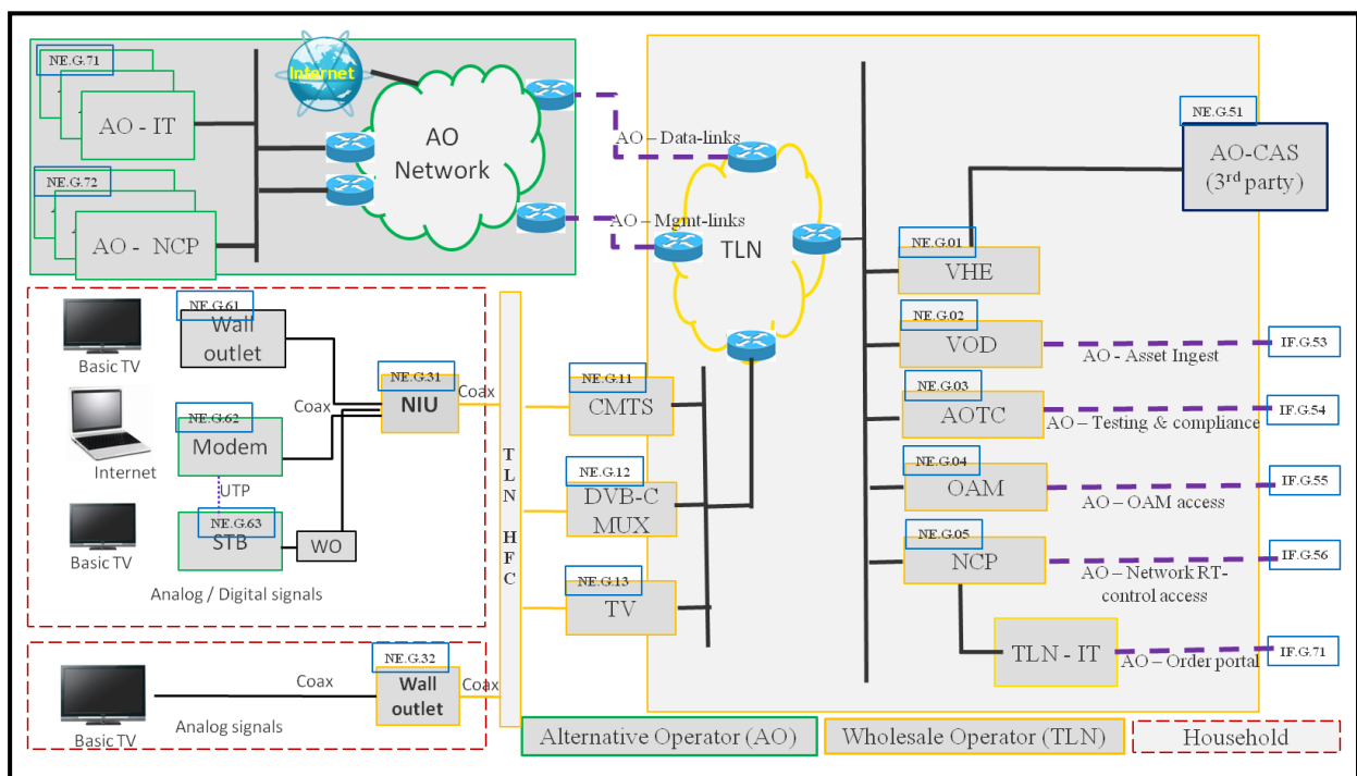
Figure 2-1: NIU Interface Ports
