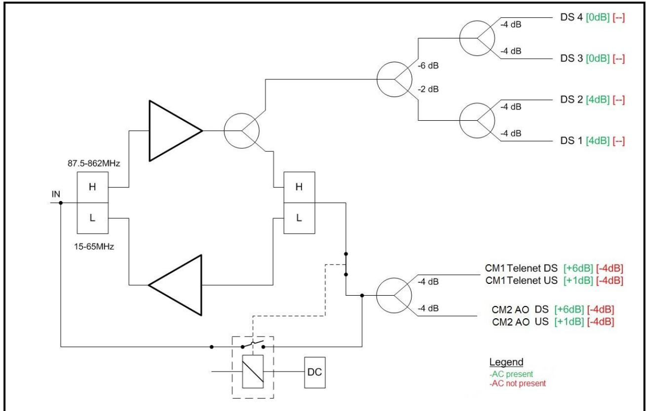
Figure 3-3: NIU RF Example
