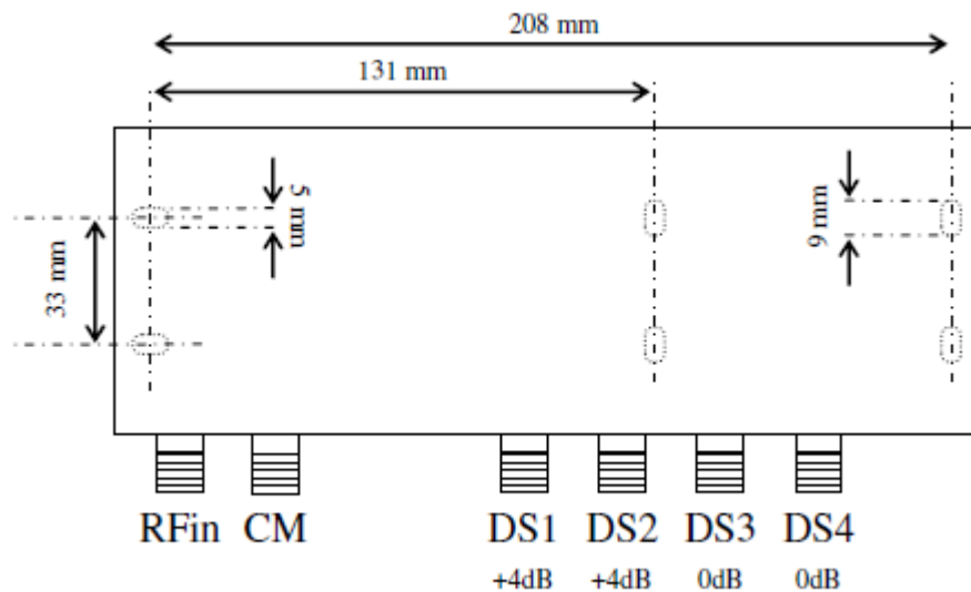
Figure 3-1: NIU Physical View
