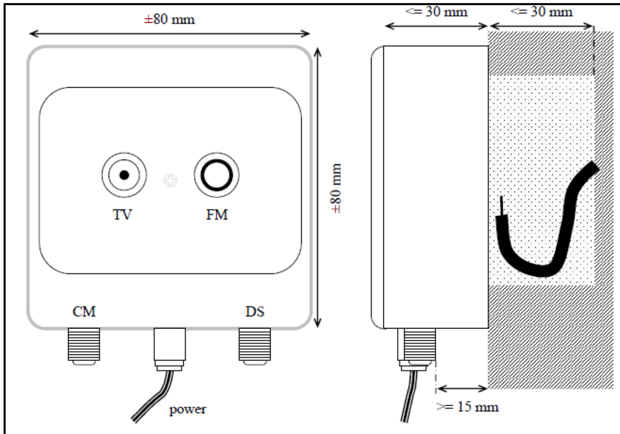
Figure 3-2: Wall Outlet
